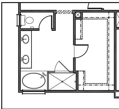
OPT MASTER BATH SECOND FLOOR
