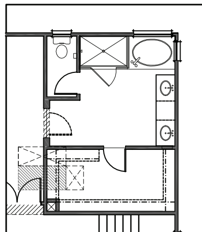
OPT MASTER BATH SECOND FLOOR
